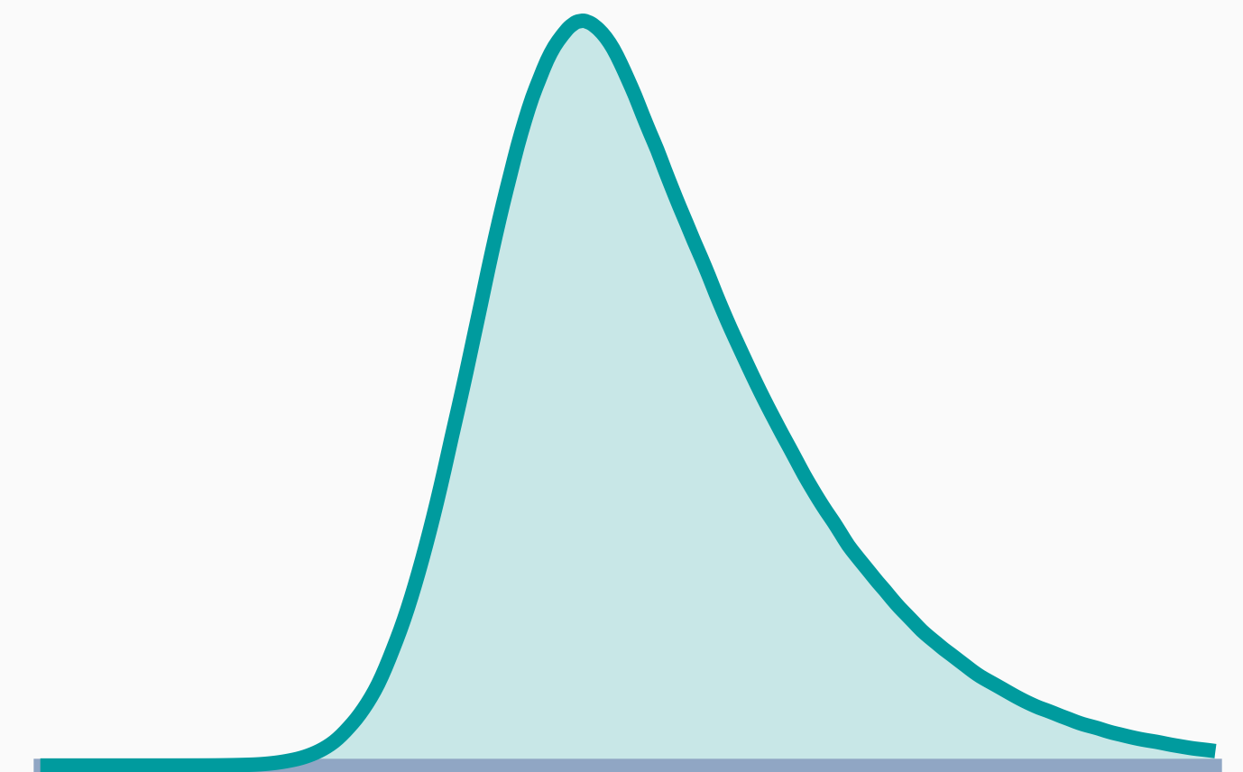
Positively Skewed
