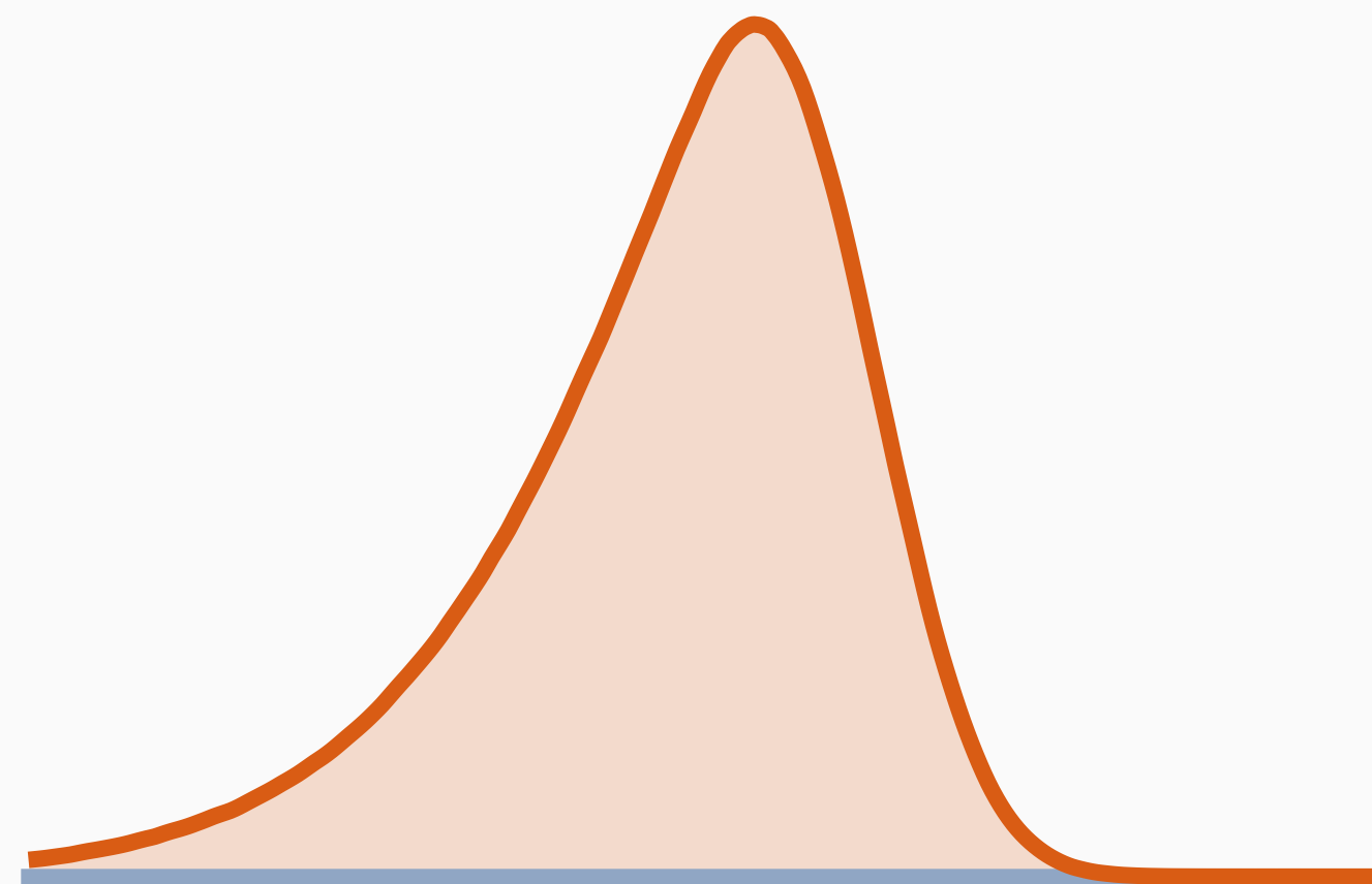
Negatively Skewed
